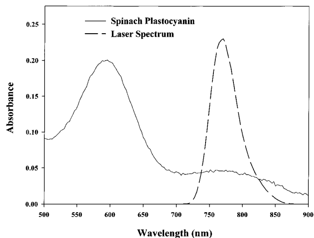
Figure 1. Absorption spectrum of spinach plastocyanin and the laser spectrum used in the pump–probe measurements. The absorption band at \sim 600 \text{ nm} is the ligand-to-metal charge-transfer transition, while the band centered at \sim 770 \text{ nm} is a combination of three d \rightarrow d transitions of the blue copper atom.
